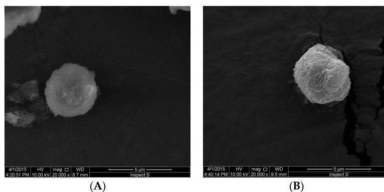
Figure 3. Representative SEM images of S-SEDDS microparticles: (A) formulation OF2; (B) formulation CF3 (magnification 20,000×).
