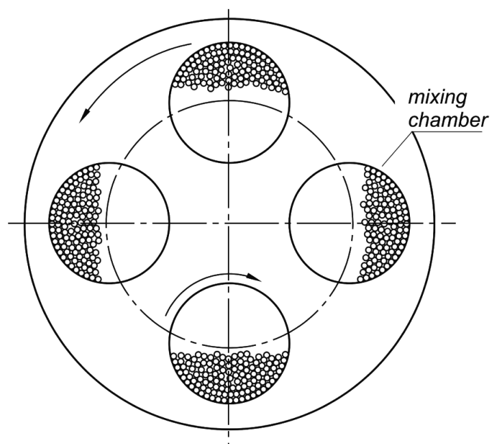
Fig. 2. Schematic representation of planetary ball mill
