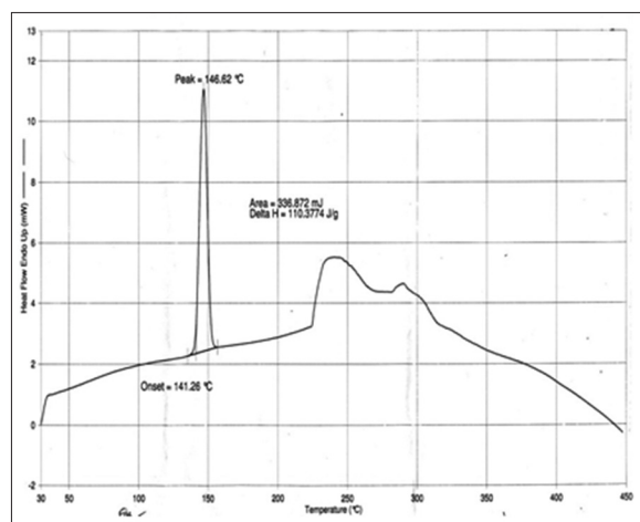
Figure 4: Differential scanning calorimetry thermograms of formulation F2
