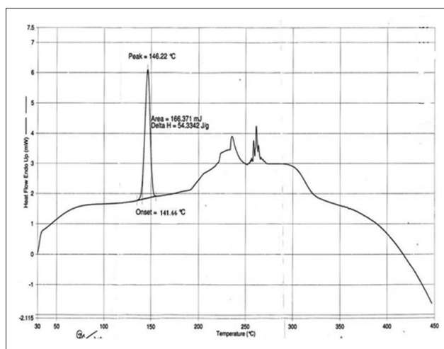
Figure 5: Differential scanning calorimetry thermograms of formulation F8
