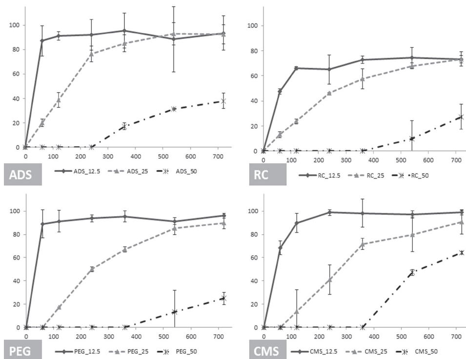
Fig. 5. Dissolution profiles of glucose pellets with different composition and coating concentration. The full line (—) represents 12.5 % coating, the dashed line (---) represents 25 % coating, and the dash-dot line (- · -) represents 50 % coating.
