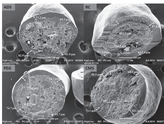
Fig. 4. SEM images of cut pellets. Standard numbers identify the coating thickness, underlined numbers identify the total pellet length.
