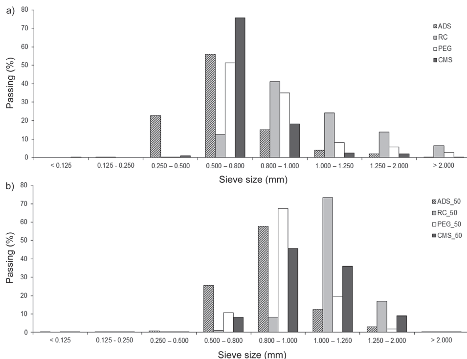
Fig. 1. Sieve analysis of: a) cores and b) coated pellets (50 % coating). Hatched column represents the ADS sample, light grey column represents the RC sample, white column represents the PEG sample and dark grey column represents the CMS sample.
