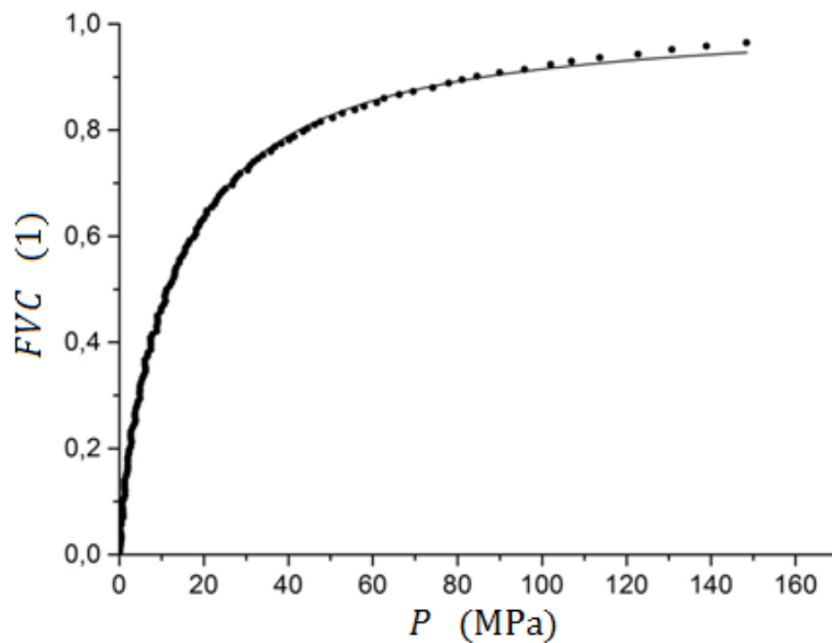
Fig. 18 Cooper-Eaton plot of the MCC Avicel PH 102
