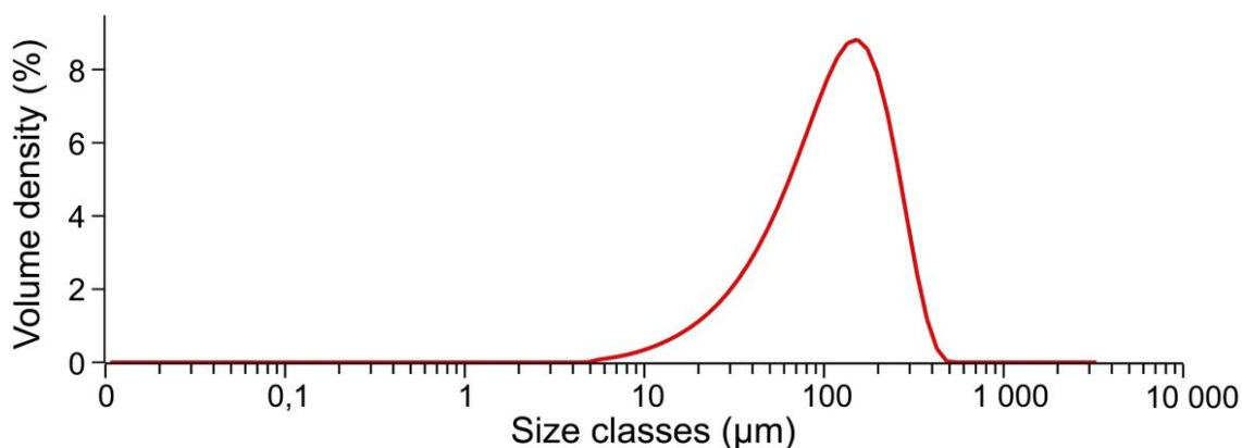
Fig. 7 Particle size distribution of MCC Avicel PH 102 measured by Malvern Mastersizer 3000
