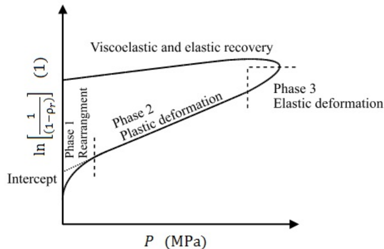
Fig. 3 A typical Heckel plot
