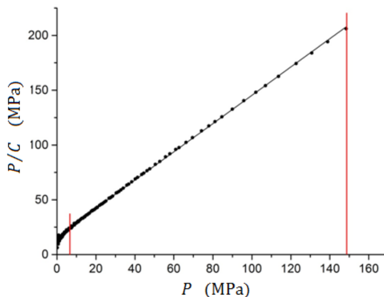
Fig. 17 Kawakita plot of the MCC Avicel PH 102
