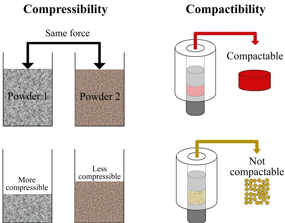
Fig. 2 Examples of compressibility and compactibility
