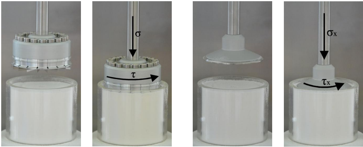
a) b) Fig. 11 Shear cell test a) shear cell head, b) principle of shear cell test
