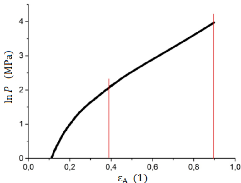
Fig. 19 Adams plot of the MCC Avicel PH 102
