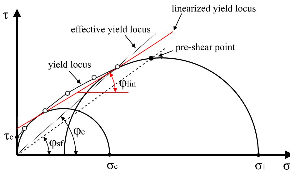
Fig. 10 An illustration of different flow parameters obtained from the shear cell test
