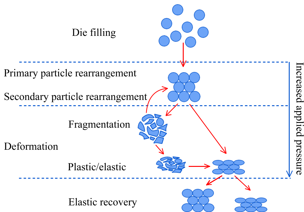
Fig. 1 Schematic illustration of the powder compression cycle
