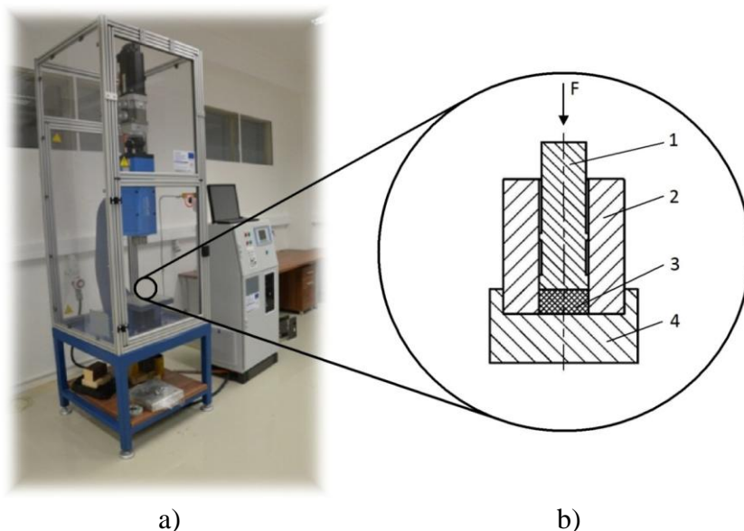
Fig. 15. Experimental station
