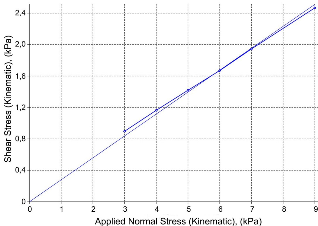
Fig. 14 Graphical result of the Wall friction test (FT4 Powder Rheometer)
