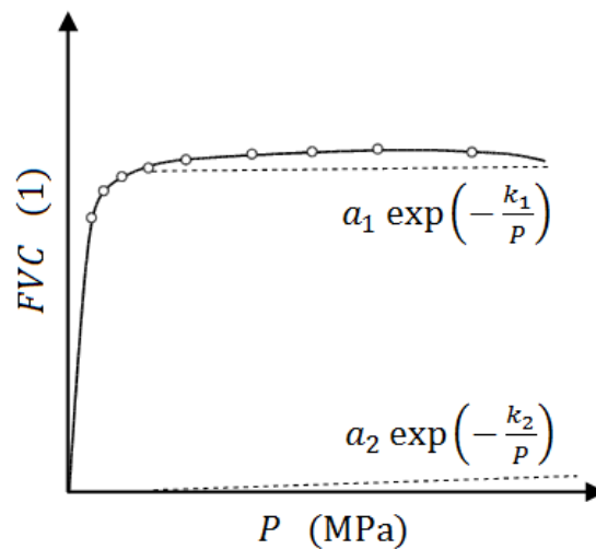
Fig. 5 A typical Cooper - Eaton plot
