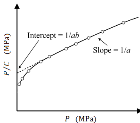
Fig. 4 A typical Kawakita plot
