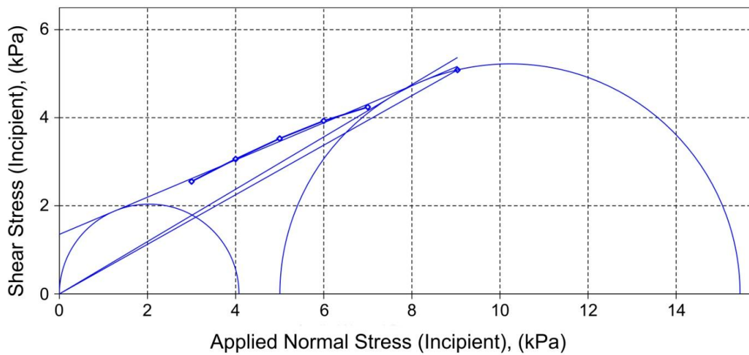
Fig. 13 Graphical results of the Shear test (FT4 Powder Rheometer)
