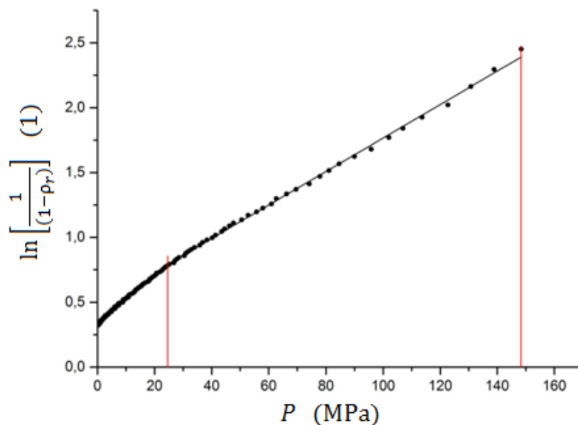
Fig. 16 Heckel plot of the MCC Avicel PH 102
