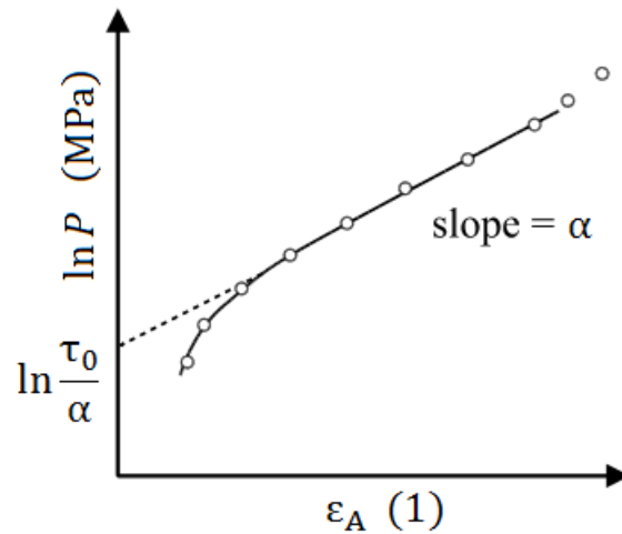
Fig. 6 A typical Adams plot
