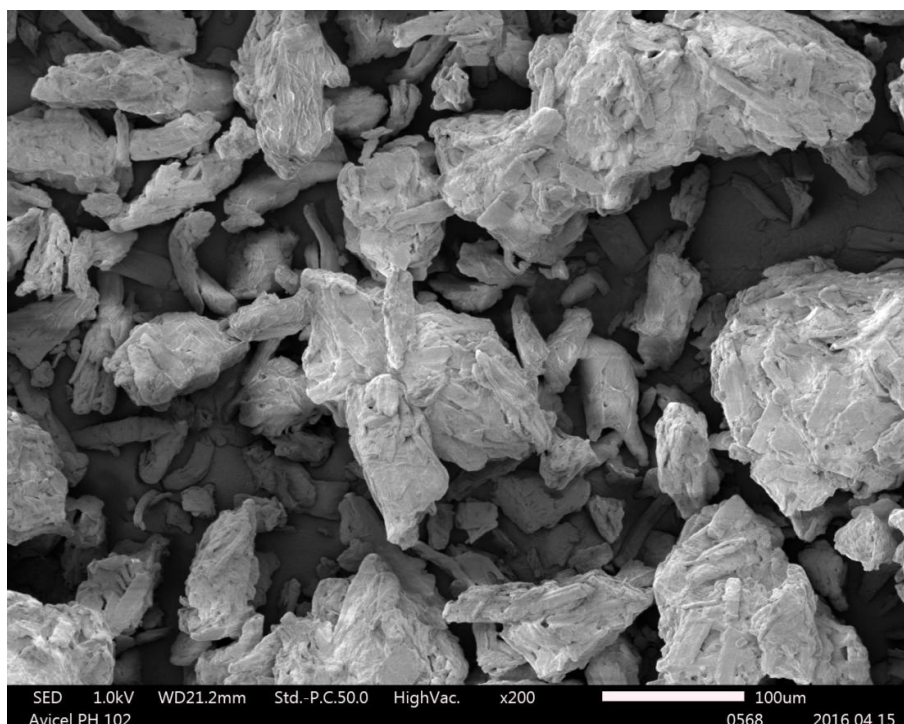
Fig. 8 Electron microscopy image of the bulk powder MCC Avicel PH 102
