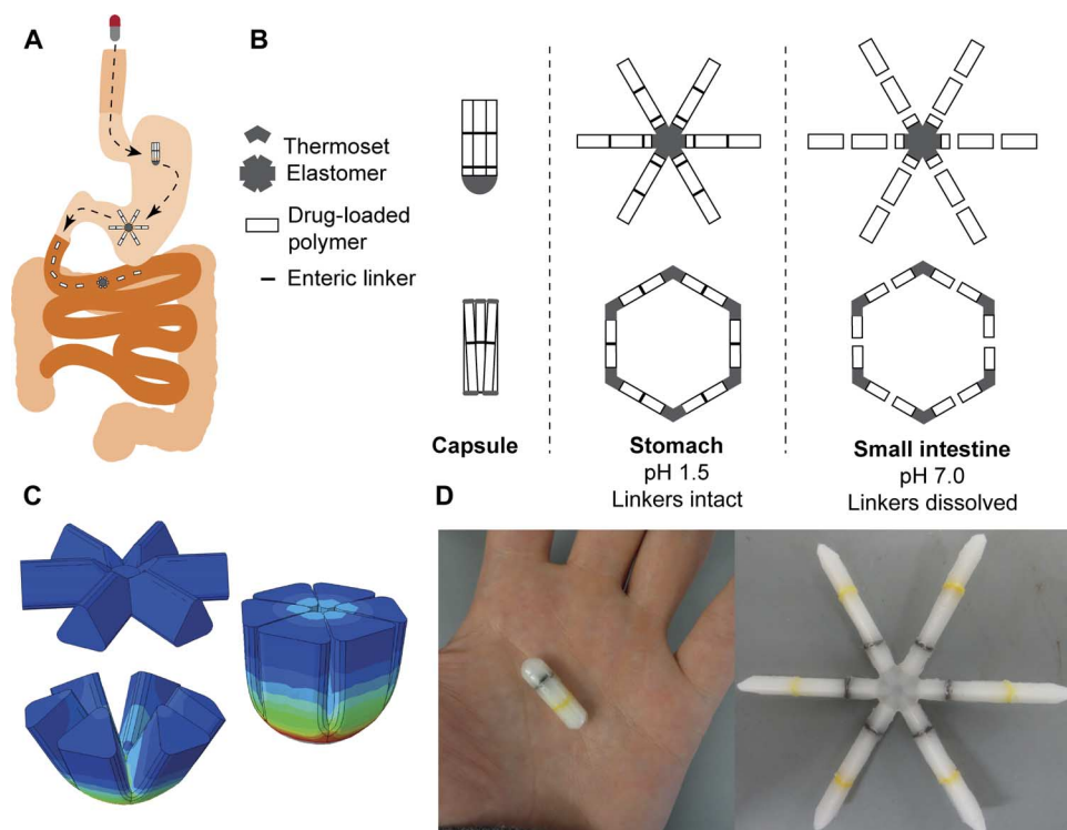
Fig. 1. Design of a modular gastric residence vehicle. (A) Schematic of deployment of gastric residence drug delivery dosage form via ingestible capsule. (B) Two families of geometric arrangements of flexible and rigid elements able to fit into a capsule and method of dissolution via fracture at designed failure points in presence of intestinal pH. Schematic enteric linkers, such as those evaluated in vitro (see fig. S3), are represented by black lines. (C) Stress distribution of the flexible element when it is folded into the capsule, generated with the finite element method. (D) Representative dosage form after assembly and loading into a 00el gelatin capsule. Linkers, such as those evaluated in vitro in fig. S3, are yellow and black.
