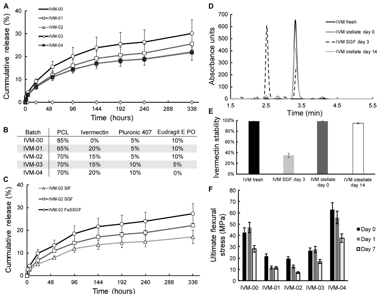
Fig. 3. In vitro release and stability of ivermectin. (A) In vitro release of ivermectin (IVM) from drug-loaded stellate dosage forms with different formulations in SGF. (B) Summary of formulations used for in vitro release and mechanical testing, as in (A) and (F), respectively. (C) In vitro release of ivermectin in SGF, SIF, and fasted-state SGF (FaSSGF). (D) Representative high-performance liquid chromatography (HPLC) curves of ivermectin degradation after 3 days in SGF and of ivermectin stabilized in PCL and incubated in SGF for 0 and 14 days. (E) Ivermectin stability when homogeneously dispersed in a PCL matrix versus in a solution after incubation in SGF (an acidic environment) over 14 days. (F) Flexural strength of drug-polymer blends after incubation in SGF for days 0, 1, and 7. Error bars represent SD for n = 3 samples in each group.
