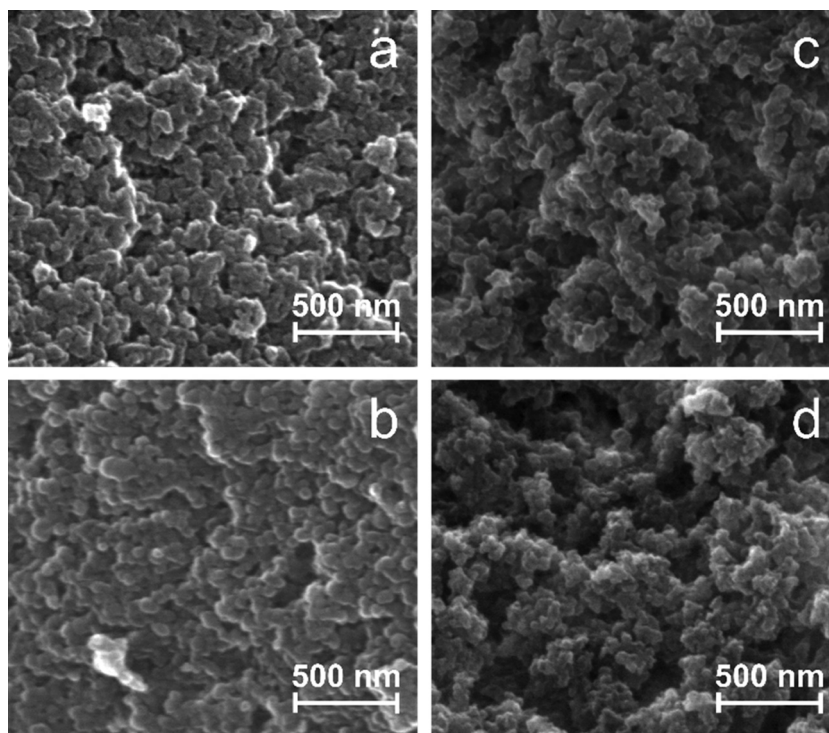
Fig. 3. SEM micrographs of the interior of the HP-DA (a), HP-DB (b), CP-DA (c) and CP-DB (d) Composites.
