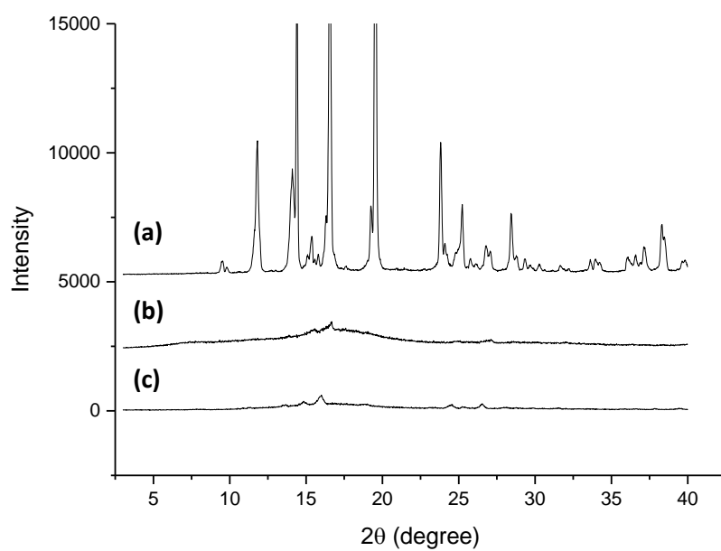
Figure 4 - XRD of (a) pure isoniazid; (b) 20% w/w Eudragit E-PO/isoniazid extrudate; (c) 30% w/w Eudragit E-PO/isoniazid extrudate.
