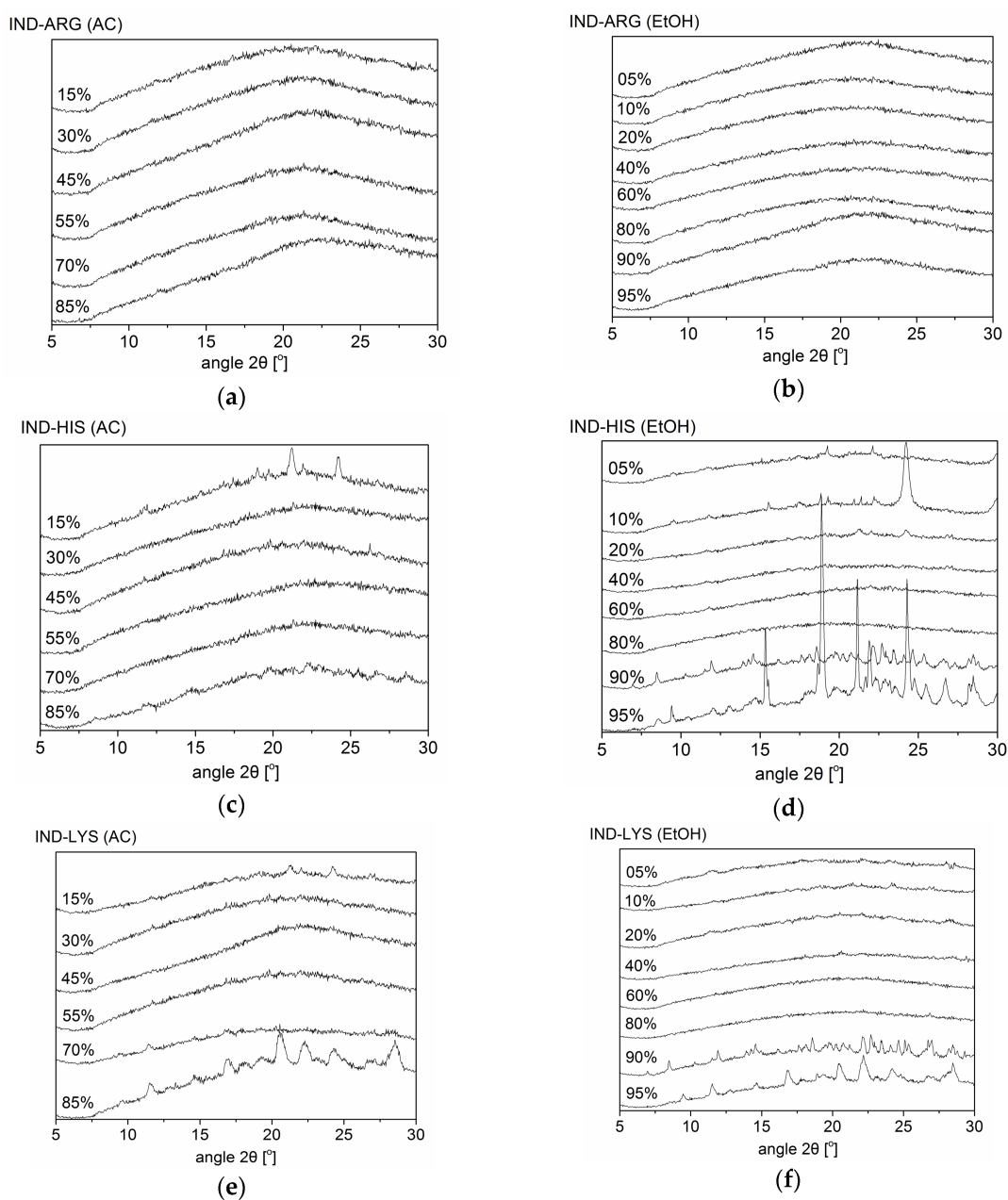
Figure 2. XRPD diffractograms of indomethacin–arginine (IND–ARG), IND–histidine (IND–HIS) and IND–lysine (IND–LYS) mixtures prepared by spray-drying (SD). Organic solvent denoted in percentage (%) is acetone (AC) in (a,c,e); and ethanol (EtOH) in (b,d,f).
