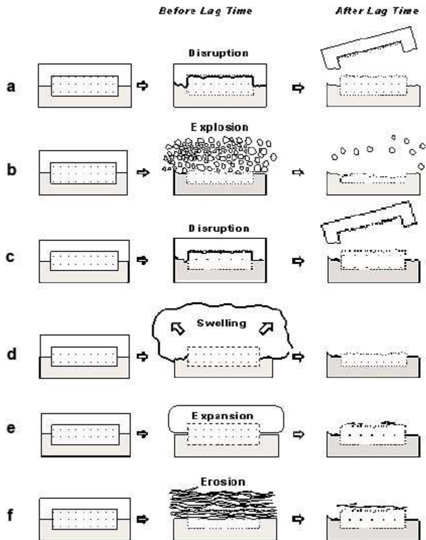
FIGURE 2 : schematic dissolution process for drug release from compression-coated tablets containing the same lower compression-coat (ethylcellulose coarse powder) and different upper compression-coats: (a) ec coarse powder and ec fine powder = 6:1; (b) ethylcellulose coarse powder and explotab = 6:1; (c) ec coarse powder and avicel = 6:1; (d) ethylcellulose coarse powder and hydroxypropylmethyl-cellulose = 6:1; (e) ethylcellulose coarse powder and spray dried lactose = 6:1; (f) ethylcellulose coarse powder and dibasic calcium phosphate = 6:1 [16] .
