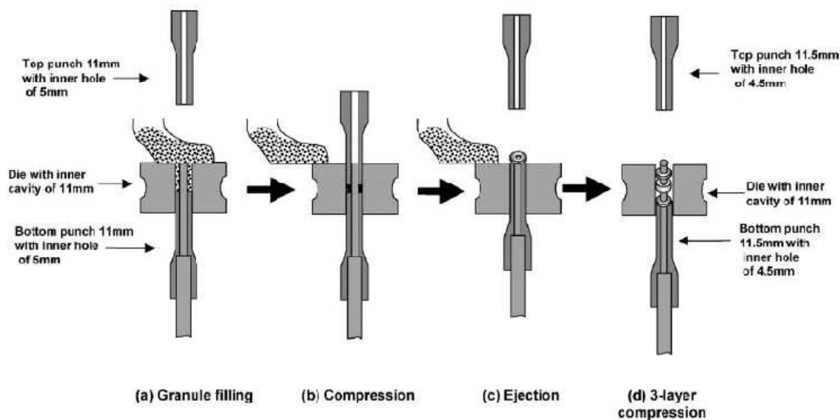
FIGURE 5 : SCHEMATIC DIAGRAM OF THE PROCESS OF THREE-LAYERED TABLETS ON THE MANESTY-F3 TABLETING PRESS.
