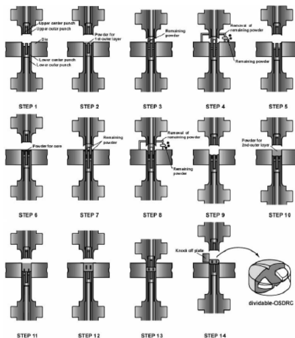
FIGURE 4 : MANUFACTURING PROCESS OF DIVIDABLE OSDRC
