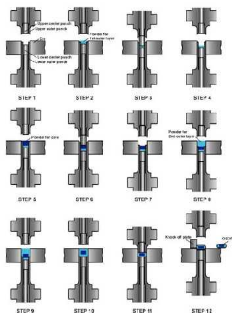
FIGURE 3 :PROCESS OF OSDRC MANUFACTURING METHOD AS DESCRIBED.
